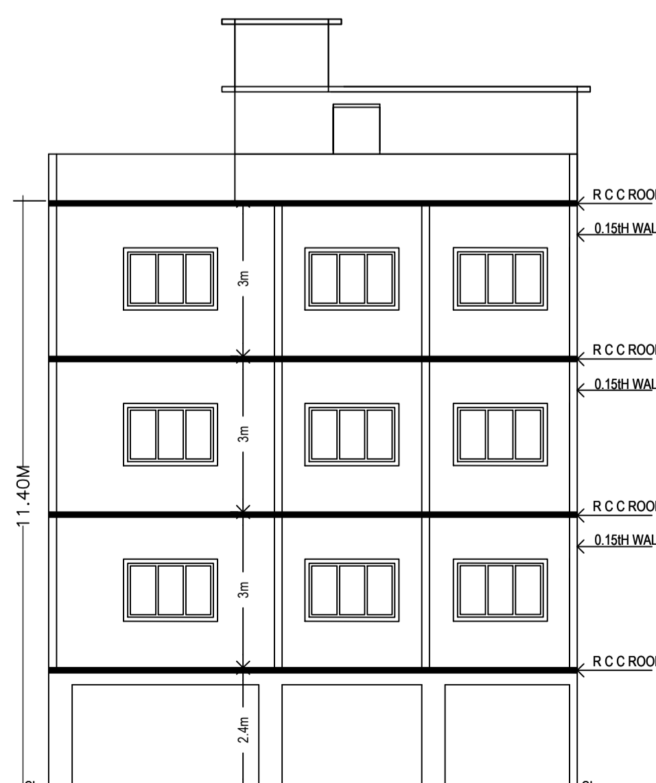
SECTION @ X-X
